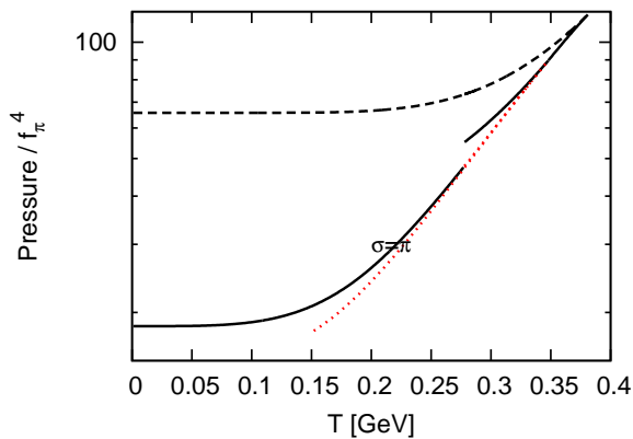
FIG. 11: The same as in Fig. 9 but for the pressure.
