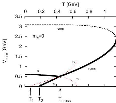
FIG. 4: Meson masses of Fig. 1 but in wider temperature region. The upper metastable branch is displayed by the long-dashed line.
