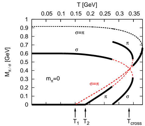
FIG. 9: Meson masses as functions of temperature for \mu = 300 MeV and m_{\pi} = 0 case. Stable branches are presented by solid lines, whereas metastable ones – by dashed lines.
