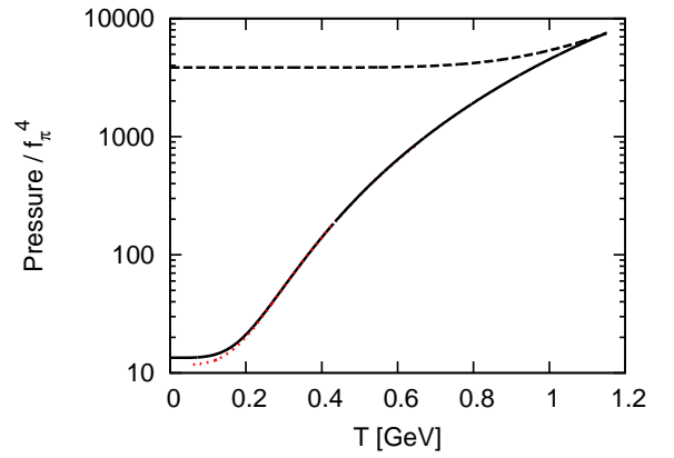
FIG. 5: The same as in Fig. 4 but for the pressure.
