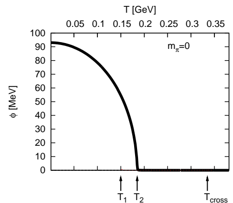
FIG. 10: The same as in Fig. 9 but for the field \phi .
